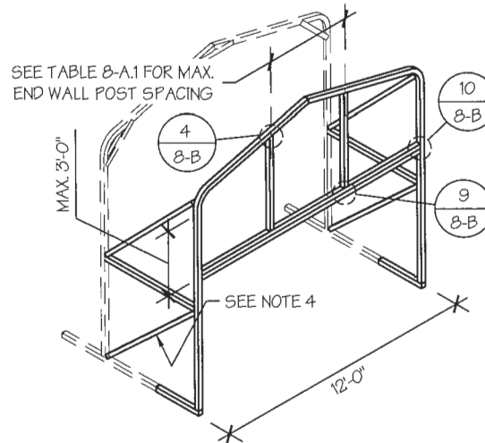
PARTIAL END WALL FRAMING SCALE: NTS
