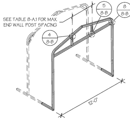
END WALL GABLES SCALE: NTS
