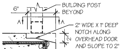
OVERHEAD DOOR NOTCH DETAIL SCALE: NTS
