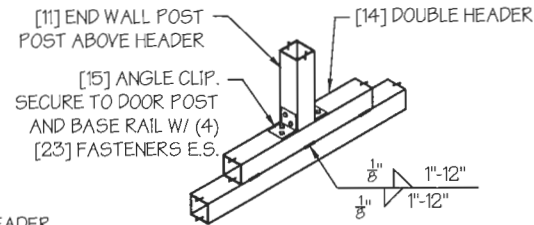
END WALL POST ABOVE DOUBLE HEADER CONN. DETAIL SCALE: NTS
