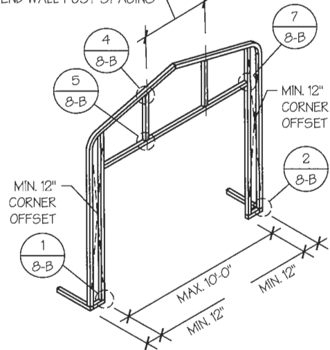
END WALL OVER HEAD DOOR OPENINGS SCALE: NTS
