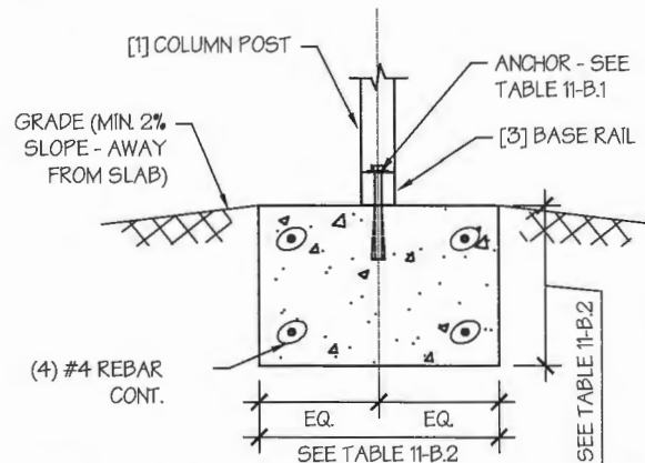
CONCRETE STRIP FOUNDATION DETAIL
